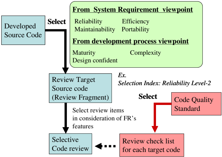
Fig. 4. Overview of the proposed process (SRP)
