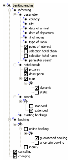
Fig. 10. Product Configuration (modeled with fmp [1])
