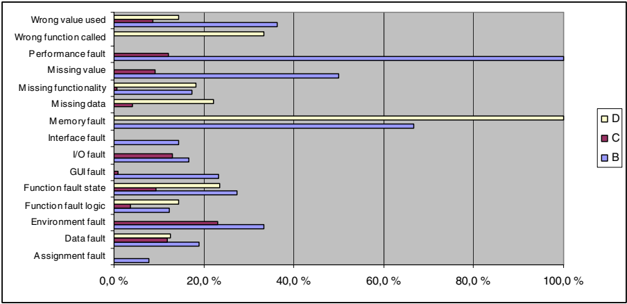
Fig. 1. Percentage of high severity faults in some fault categories
