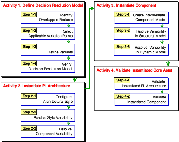
Fig. 3. Process to Instantiate Core Assets
