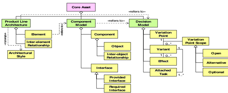
Fig. 1. Meta-model of Core Assets
