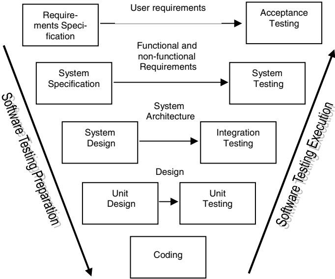
Fig. 2. The V model
