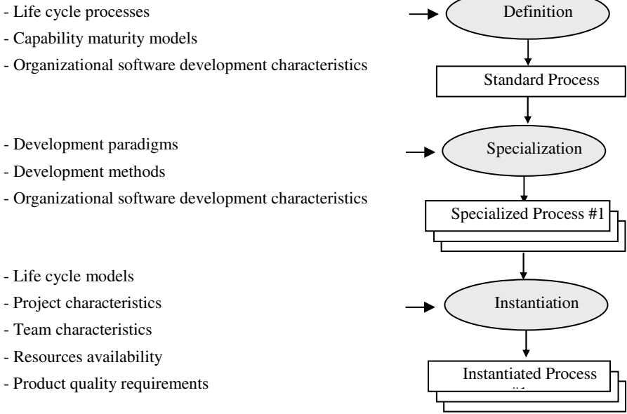
Fig. 1. Software processes definition approach
