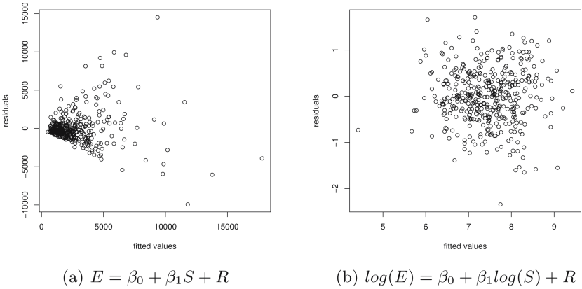
Fig. 1. Residuals of Linear Models plotted against the Fitted Values
