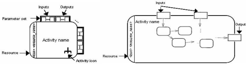
Fig. 2. Shorthand ( left ) and expanded ( right ) notation of an Activity
